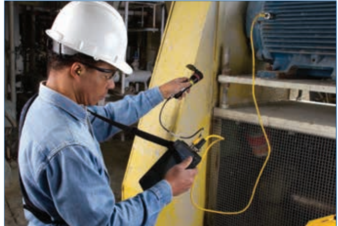
The AMS 430 Laser Speed Sensor determines shaft speed without shutting down the machine - even in extremely tight locations.
